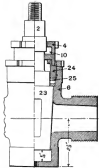
Fig. 277. Blow-off Cock.
